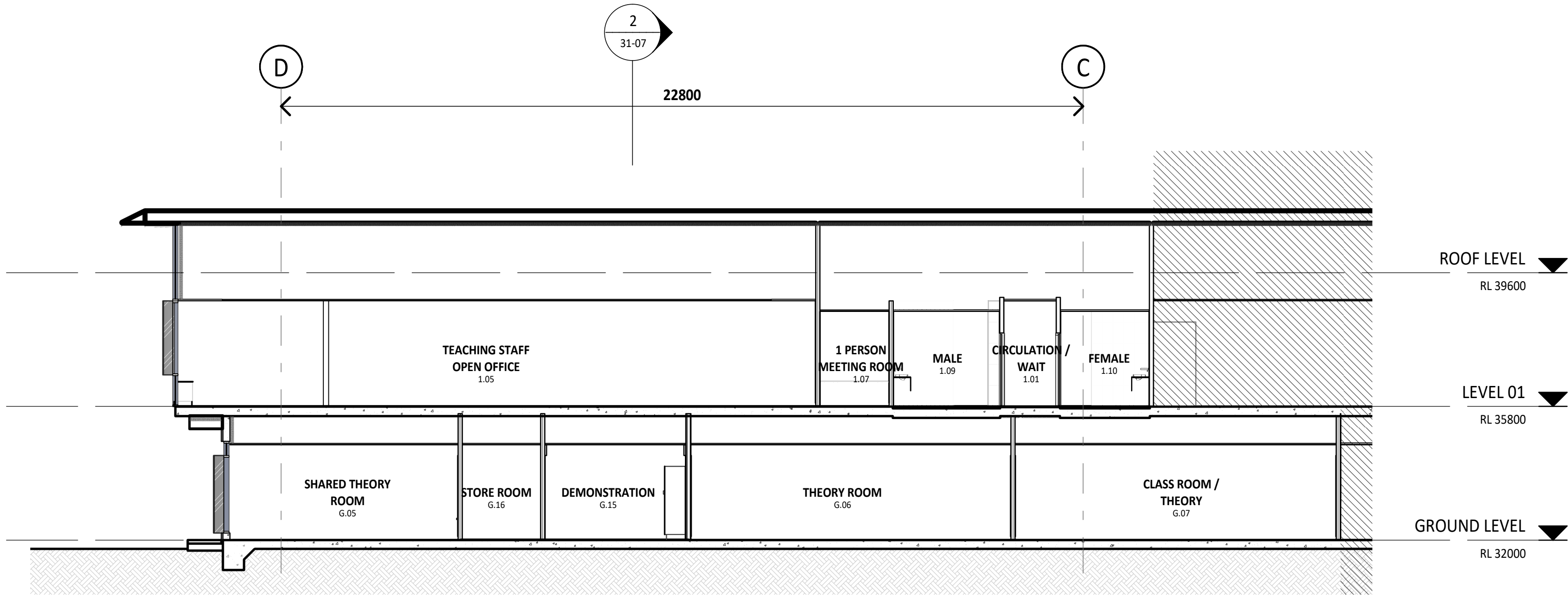
1 BUILDING SECTION - 3 - A 21-00 1 : 100
