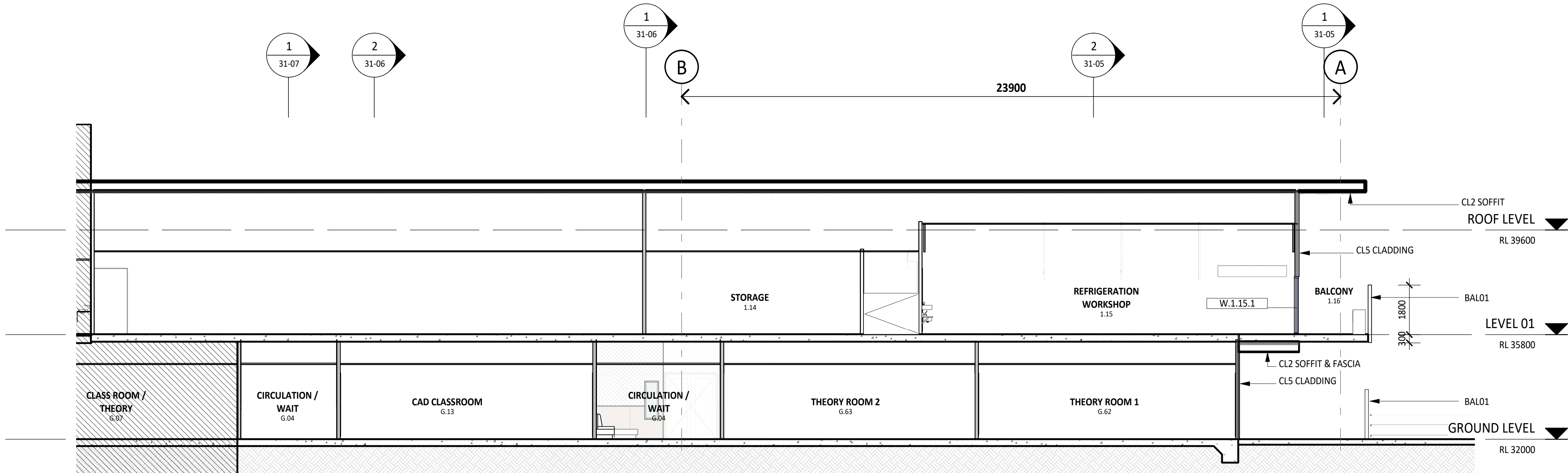
2 BUILDING SECTION - 3 - B 21-00 1 : 100
